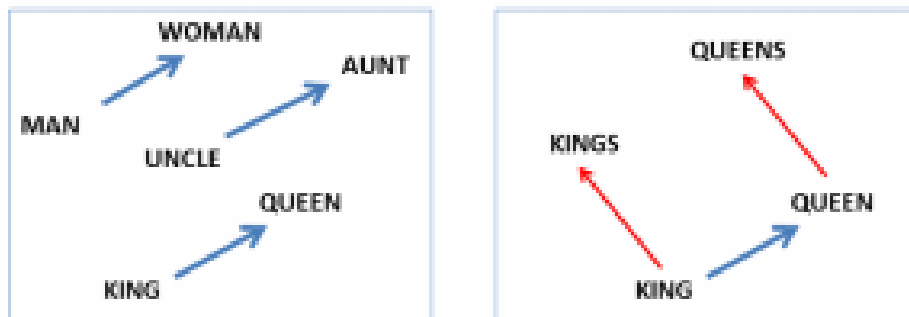
Figure 4.5. Left figure: the relationship between genders. Right figure: plural relationship between two words. Multiple relationships can be produced for a single word in high-dimensional space
