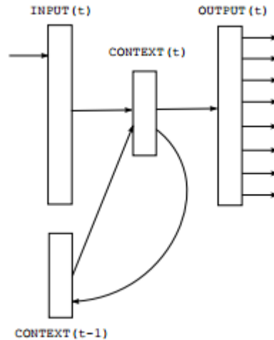
Figure 3.4. RNN-based language model
