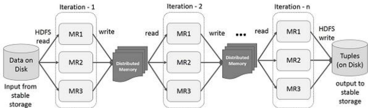
Figure 4.6. RDD architecture
