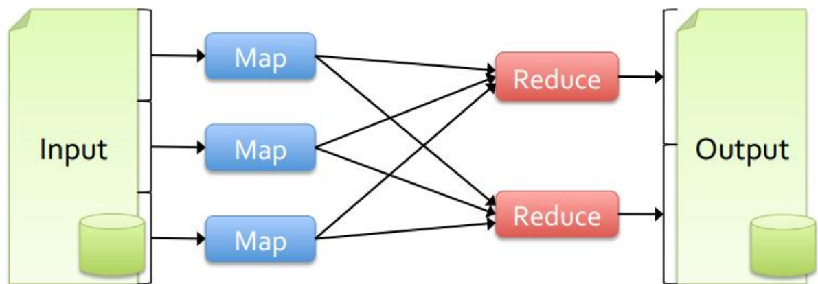
Figure 4.1. Mapreduce
