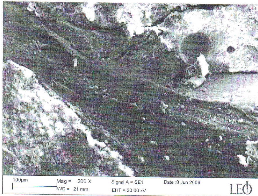
Fig. 5 Scanning electron microscopy picture of rubberized concrete
