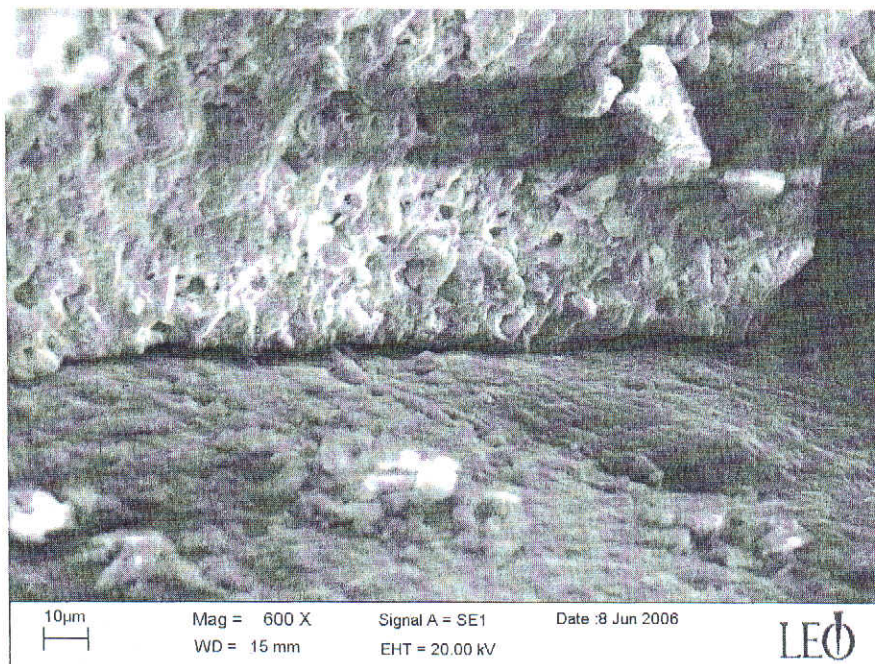
Fig. 2 ITZ between rubber and cement
