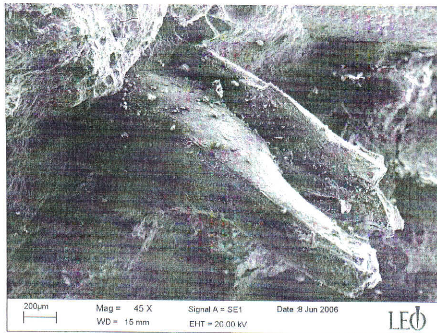
Fig. 3 SEM image of pulled out rubber tire
