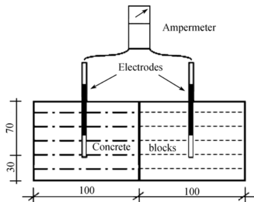
Fig. 1. Schematic demonstration of the electrodes embedded in adjacent concrete blocks (unit: mm).
