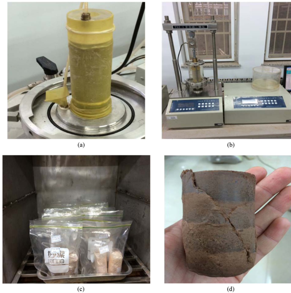
Fig. 3. Preparation of Soil Specimens for Triaxial Testing: (a) The Specimen Covered Membrane before Tests, (b) The Triaxial Compression Test System, (c) The Freeze-thaw Cabinet, (d) The Specimen after Tests
