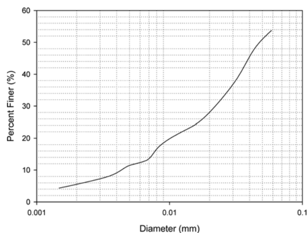
Fig. 1. Particle Size Distribution of the Studied Clayey Soil
