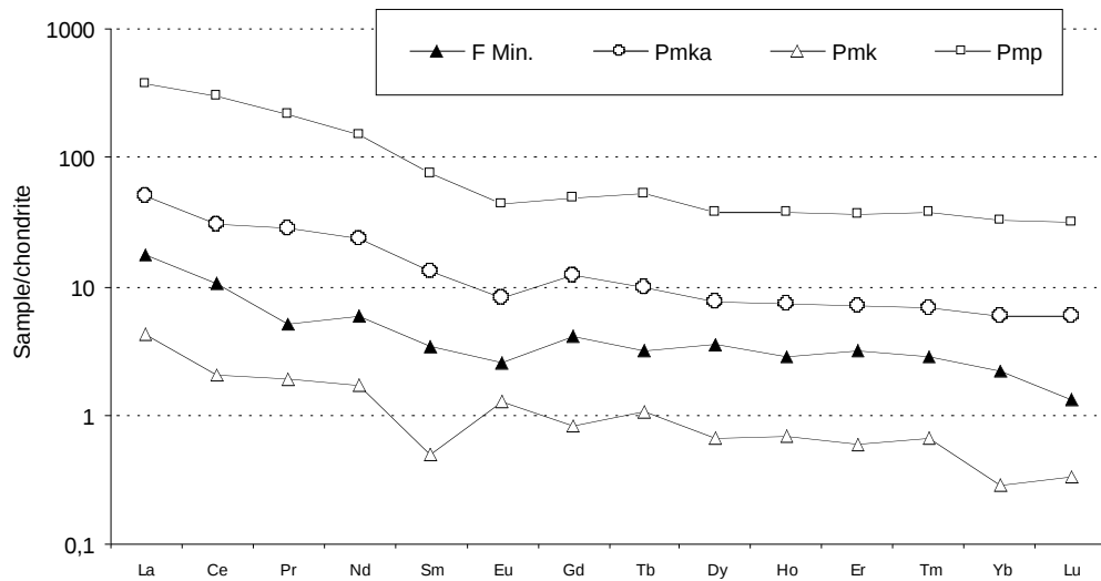
Fig. 4. Chondrite-normalized (Boynton, 1984) REE patterns of the Çelikhan fluorites and country rocks. F min: Çelikhan fluorites, Pmka: Kalecik limestone-dolomite, Pmk: Koltik limestone, Pmp: Pinarbasi formations.
