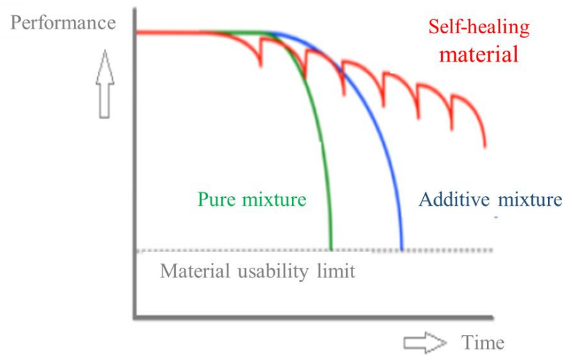
Figure 1.2. The performance-time curve in different types of material [10].
