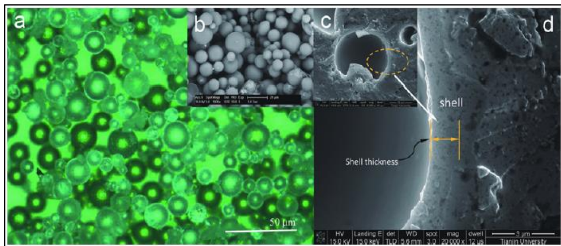
Figure 2.19. Morphologies of MF-shell microcapsules, (a) optical microscope morphology of microcapsules fabricated with core/shell ratio of 1/1 under core material stirring rate of 4000rmin -1 , (b) SEM morphology of with core/shell ratio of 1/1 under core material stirring rate of 4000rmin -1 , (c) the cross-section SEM morphology of a single microcapsule embedded in epoxy, and (d) the measurement method of shell thickness by SEM [63].
