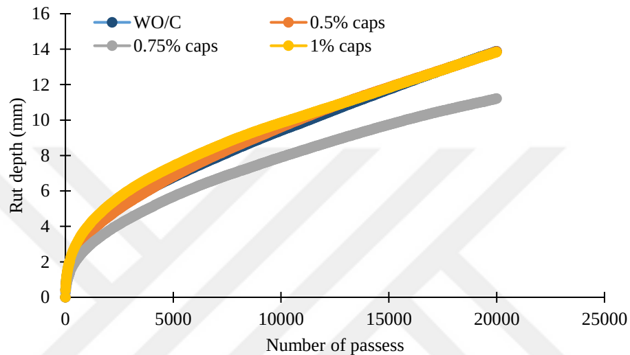
Figure 9.7. The relationship between deformation-number of load repetition obtained from the rutting test conducted at 60 °C in a dry environment.
