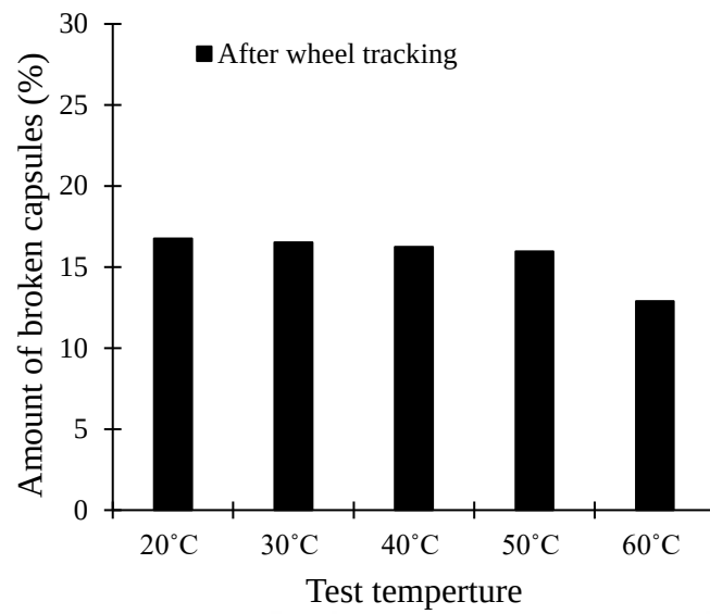
Figure 9.10. Percentage of broken capsules for mixture samples with capsules after wheel tracking tests at different heating temperatures.
