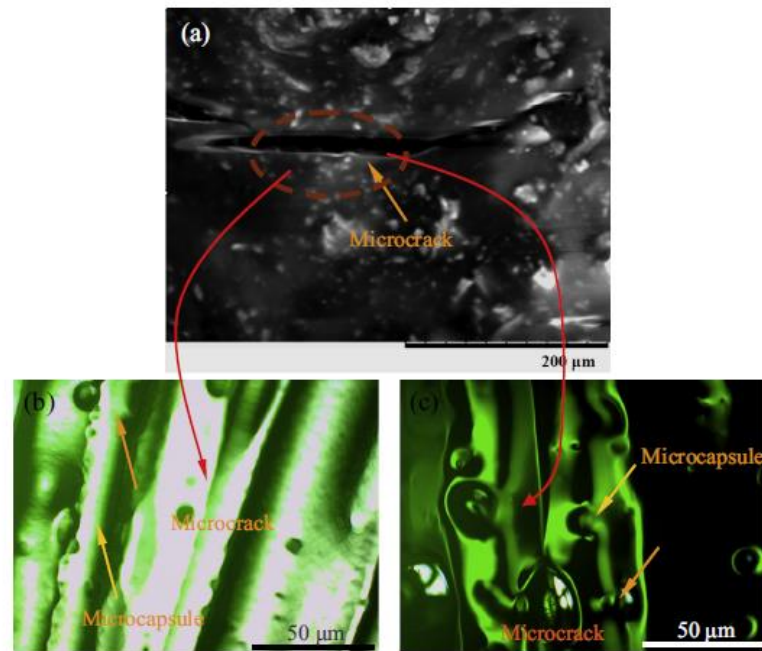
Figure 2.35. Morphologies of microcapsules in a microcrack in asphalt, (a) ESEM morphology of a microcrack, (b) fluorescence microscope morphology of microcapsules in a microcrack, and (c) fluorescence microscope morphology of microcapsules in a microcrack after 60 min [80].
