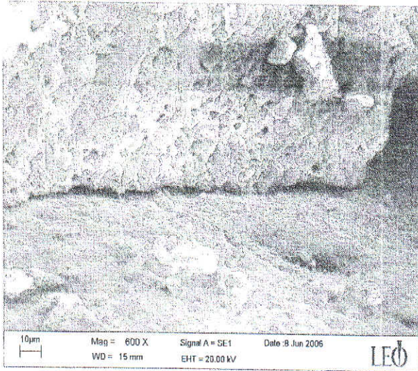
Figure 3. ITZ between rubber and cement
