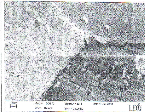
Figure 5. An image of ITZ between rubber tire, aggregate and cement paste
