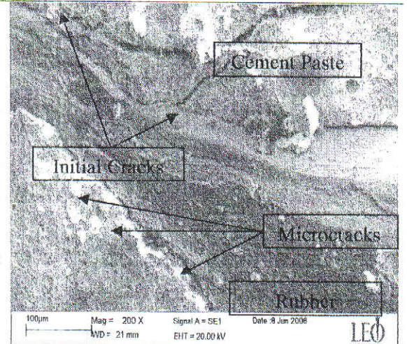
Figure 6. Scanning electron microscopy picture of rubberized concrete
