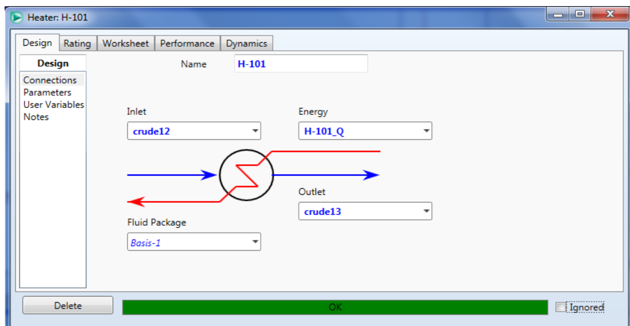
Figure 4.10 Flow diagram until the heater installation
