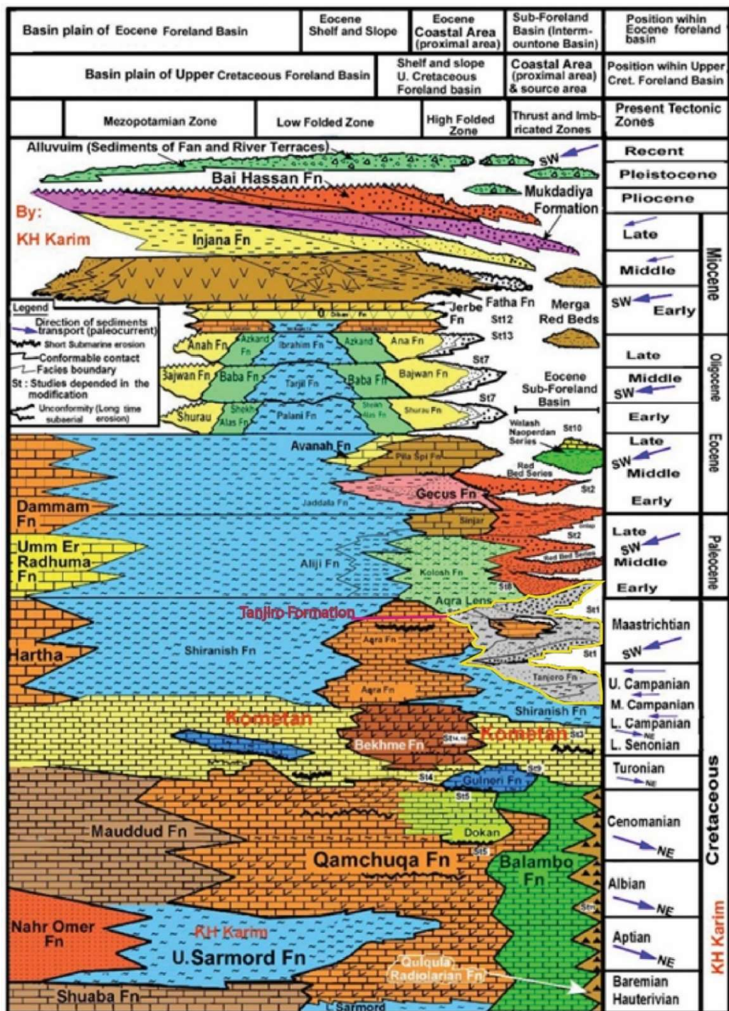
Figure 7.1. New chronostratigraphic Column of Northeast Iraq in which the stratigraphy of the Imbricated and Thrust Zones are shown and most of the previous unconformities in the High and Low Folded Zone are rejected (modified from Bellen et al, 1959 and Omeri and Sadiq, 1977). After (Karim, 2010).
