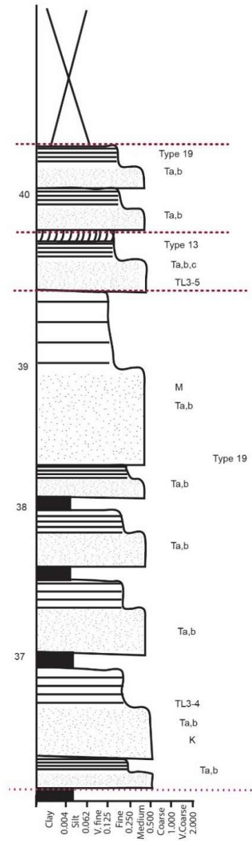
Arbat Log 3-3 (TL3-3)
