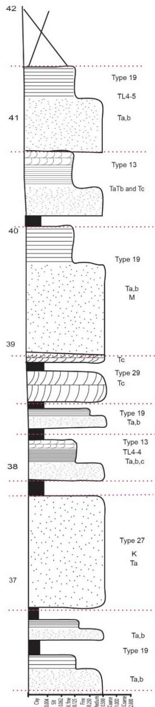
Arbat Log 4-3 (TL4-3) Vertical scale 1:25
