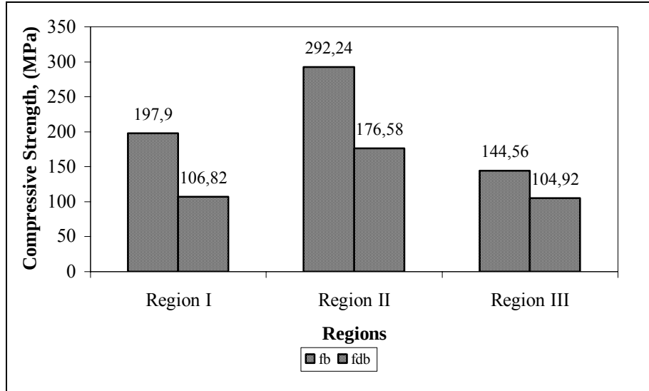
Figure 5. Compressive strength loss variations of the specimens after freeze-thaw test
