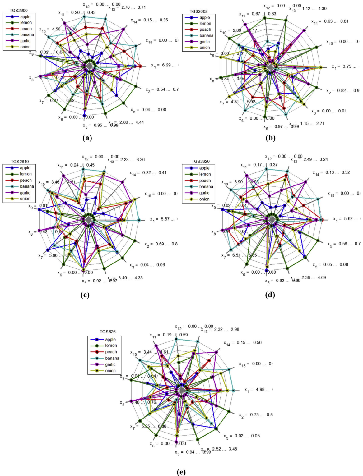
Fig. 13. The radar plots of extracted features from (a) TGS2600, (b) TGS2602, (c) TGS2610, (d) TGS2620, and (e) TGS826 for all fruit odors.
