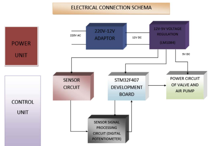
Fig. 1. Block diagram of electronic nose setup.
