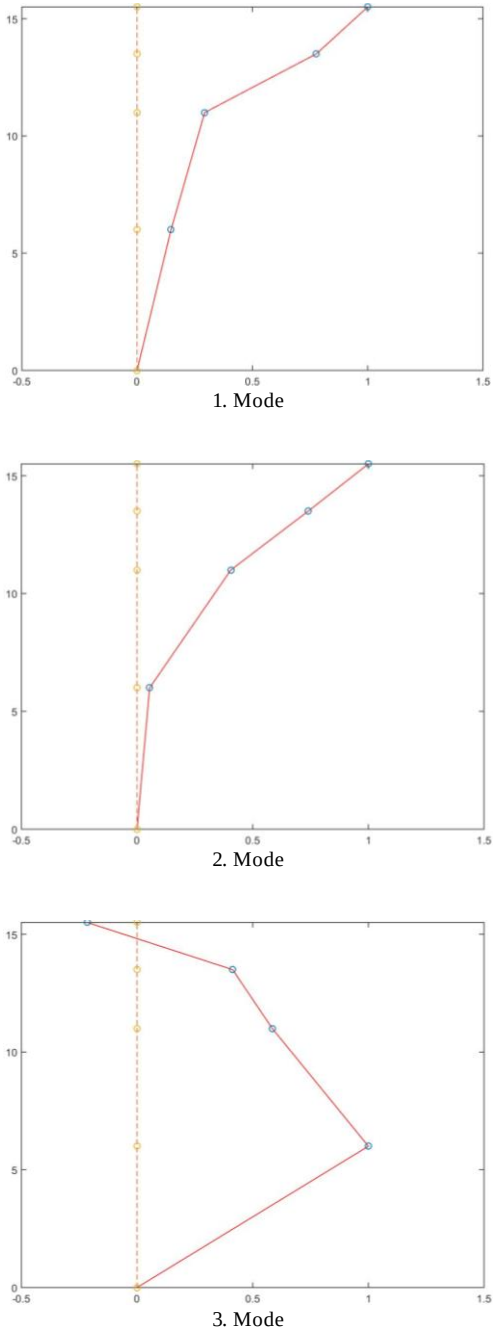
Fig. 6. Mode shapes for selected frequencies
