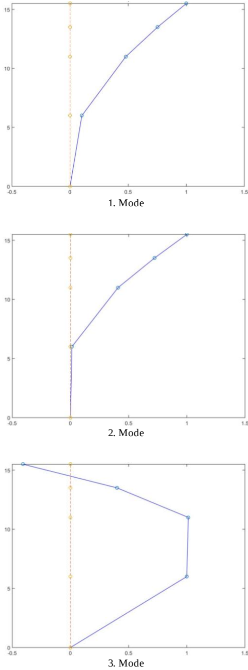
Fig. 7. The first three modes obtained using updated analytical model
