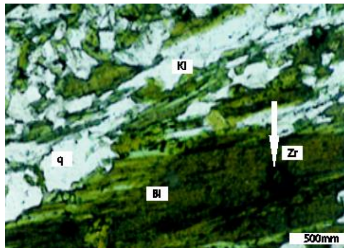
Figure 3. Metamict zircon particle inside the biotite mineral in biotite schists [5]
