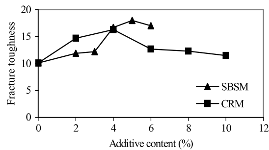
Fig. 14. Variation in fracture toughness versus additive content
